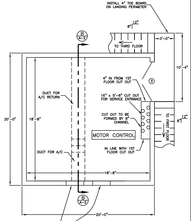
SECOND FLOOR LAYOUT (MOTOR CONTROL)
