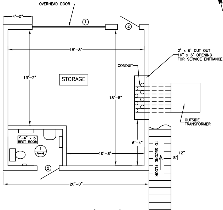
FIRST FLOOR LAYOUT (STORAGE)
