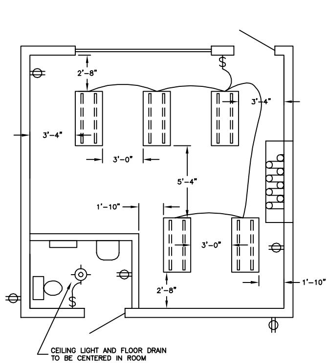
FIRST FLOOR LAYOUT (STORAGE)
